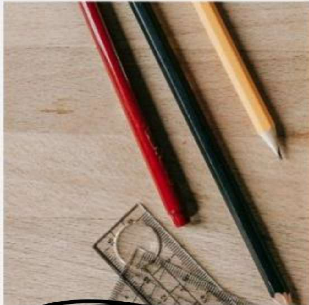
Non-Verbal Reasoning ✓
